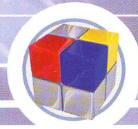
Software
